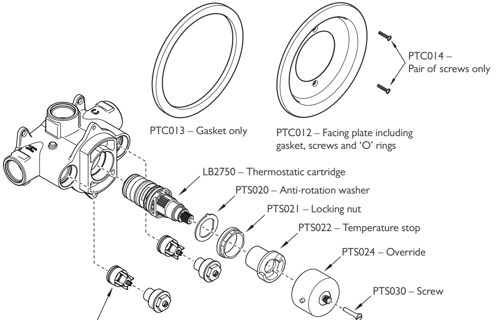
PTS034 – (FR) Ceramic ring only
